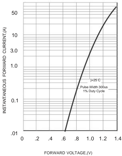
FIG.3-TYPICAL FORWARD CHARACTERISTICS
